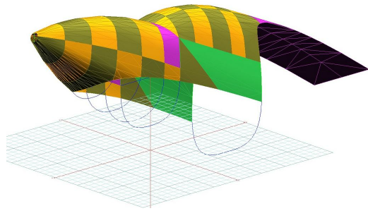
Laister LP-49 Canopy/Nose Cover, 3D model
